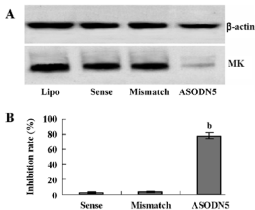
Figure 5. Analysis of MK protein expression after transfection with ASODN5, mismatch and sense. HepG2 cells were cultured in DMEM medium. A: Cell extracts were separated by SDS gel electrophoresis, transferred to a membrane, and blotted with anti-MK goat polyclonal antibody. Antiactine rabbit polyclonal antibodies was used as a loading control. B: Quantitation of the data presented in (A). Data were expressed as means±SD from four independent experiments. b P <0.05 vs the cells (CK) transfected with lipofectin alone.
