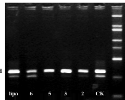
Figure 3. Effect of ASODN6, ASDON5, ASDON3, and ASDON2 on MK mRNA level. GAPDH was used as a control.
