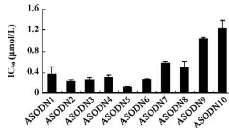
Figure 2. The IC 50 of ten ASODNs in hepatocellular carcinoma cells ( n=3 ).
